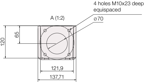
Delivery Flange Details
