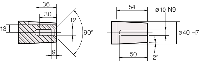
Shaft End Details
